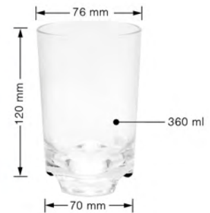
PC:10312P Tritan:10312T Material: PC or Tritan Size: 76x120mm, 360ml Package: Set 4pcs
